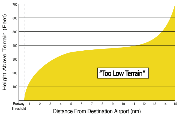
Figure 12-5 PDA Alerting Threshold
