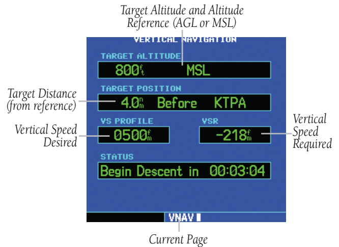
Figure 11-2 VNAV Page
