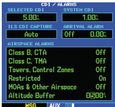
Figure 10-32 Buffer Distance Field Selected
