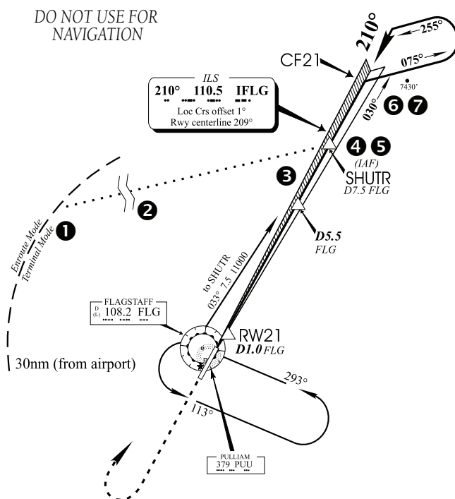
Figure 6-65 Terminal Mode
