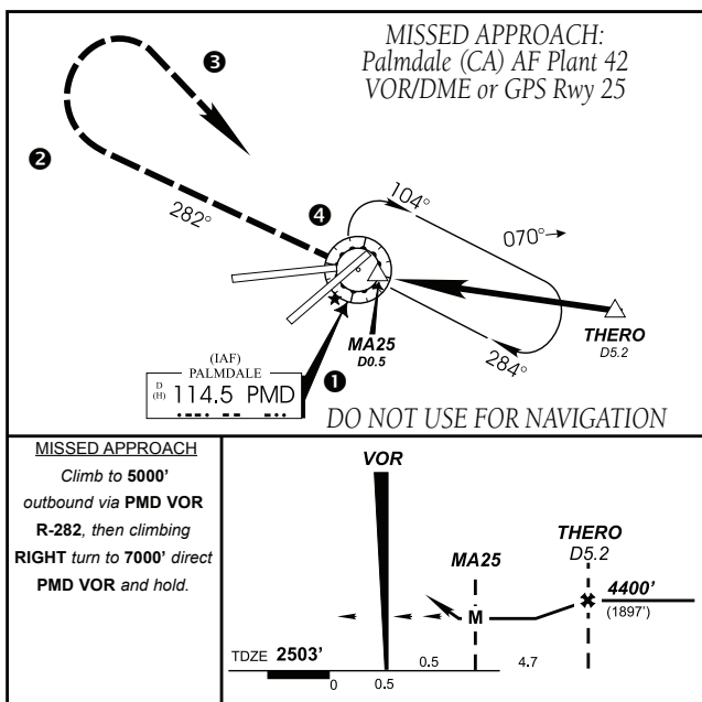
Figure 6-53 Palmdale Missed Approach
