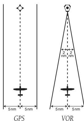
Figure C-8 CDI Comparison
