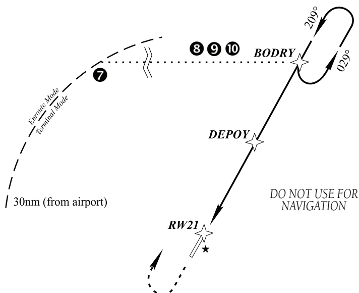
Figure 6-27 Terminal Mode
