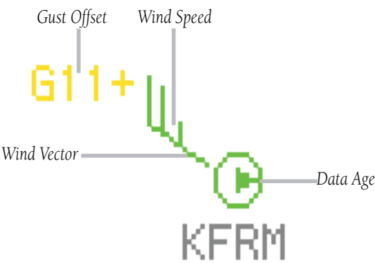
Figure 14-37 Wind Symbol
