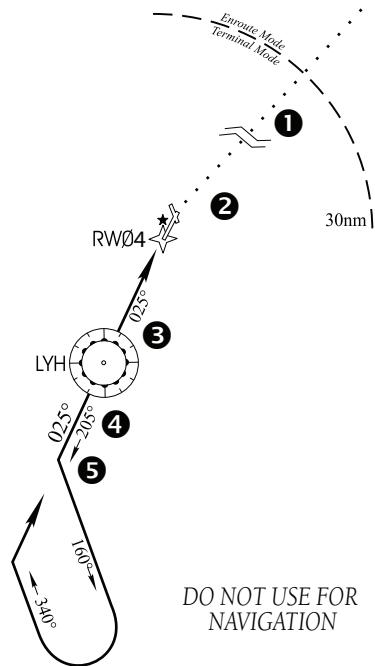
Figure 6-12 Sample Approach with Procedure Turn
