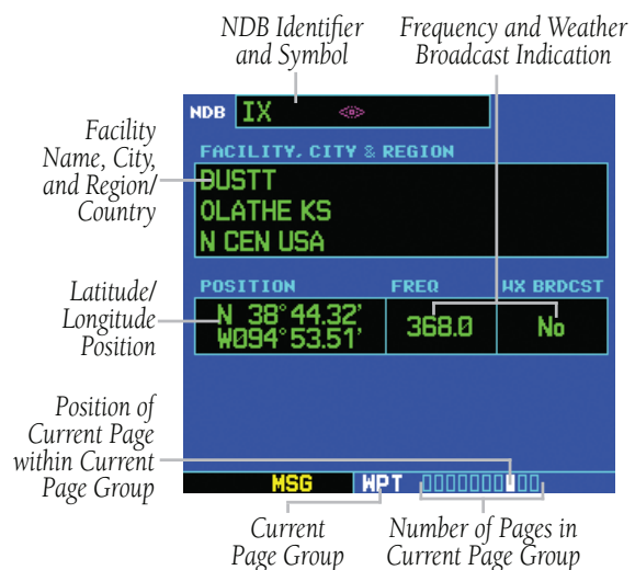
Figure 7-33 NDB Page
