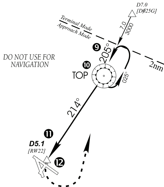
Figure 6-38 Approach Mode
