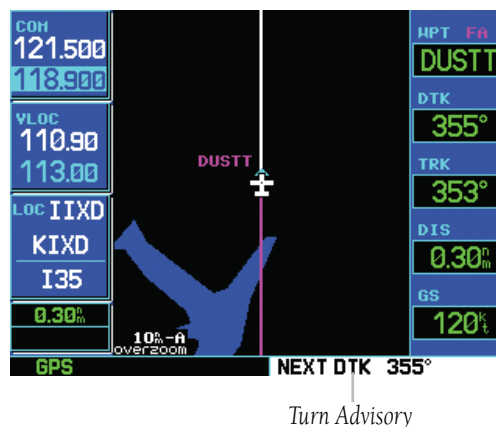
Figure 3-2 Turn Advisory
