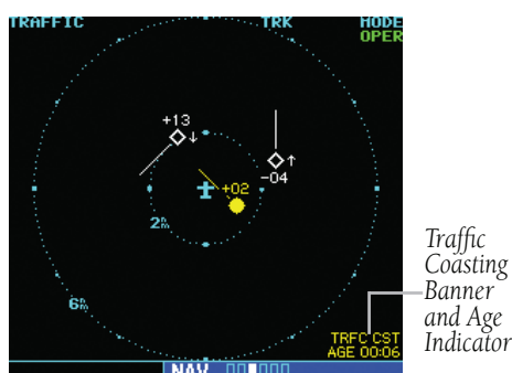
Figure 14-6 Traffic Age Indicator and Coasting Banner
