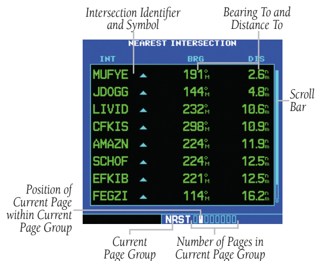
Figure 8-11 Nearest Intersection Page
