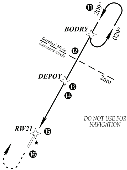
Figure 6-29 Approach Mode
