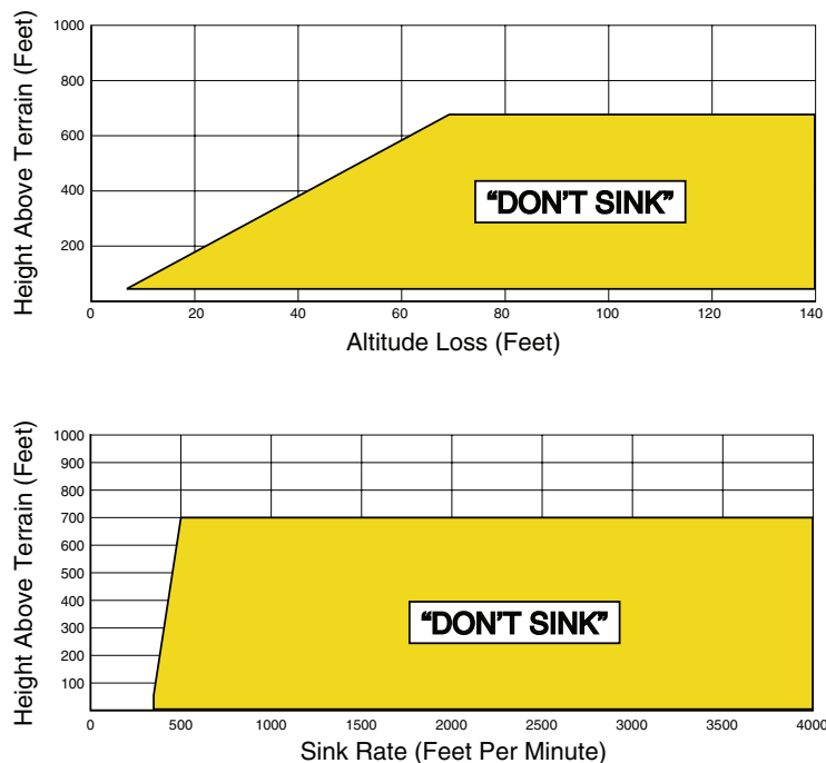
Figure 13-9 Negative Climb Rate (NCR) Alert Criteria
