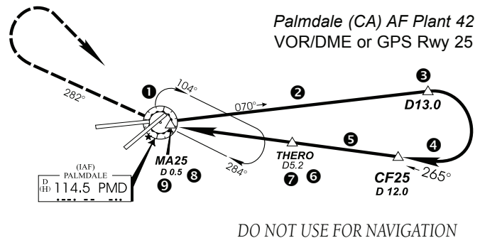
Figure 6-49 KPMD Approach
