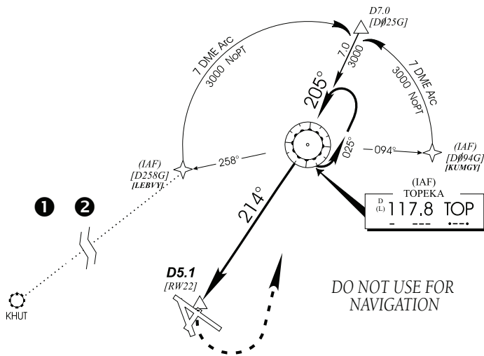
Figure 6-32 Enroute Mode
