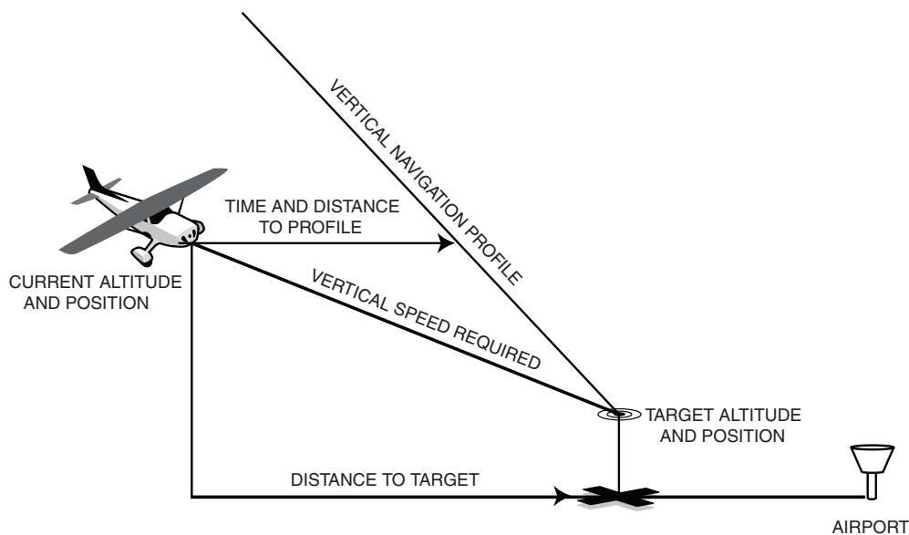
Figure 11-1 VNAV Profile
