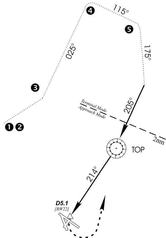
Figure 6-43 Terminal Mode
