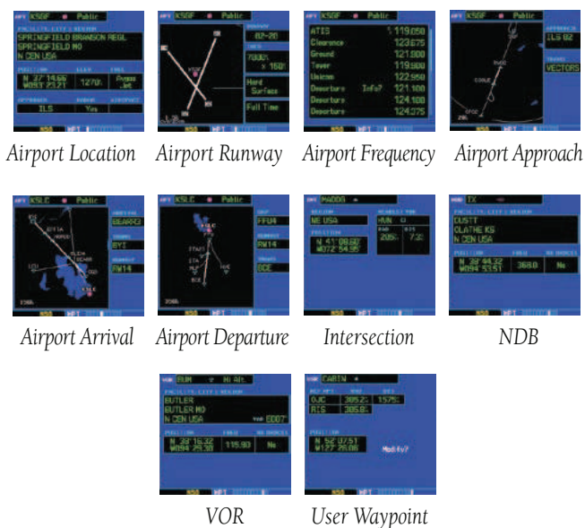
Figure 7-1 WPT Pages
