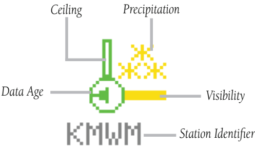
Figure 14-36 METAR Symbol
