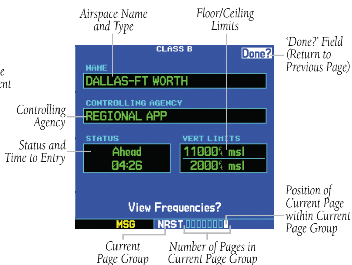
Figure 8-25 Airspace Page
