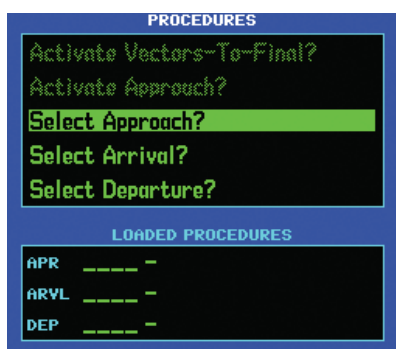
Figure 6-63 Procedures Page
