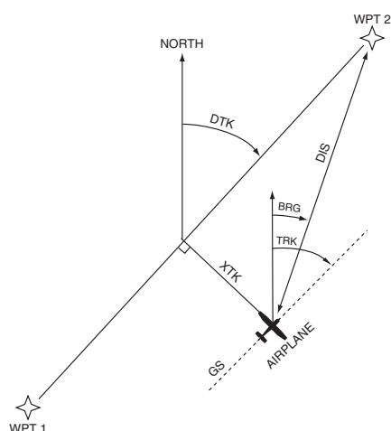
Figure 15-1 Illustrated NAV Terms
