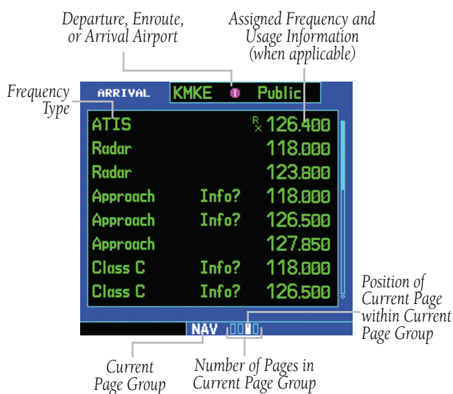
Figure 3-42 NAV/COM Page
