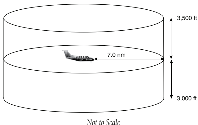
Figure 14-1 TIS Coverage Volume
