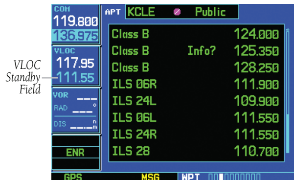
Figure 7-15 111.55 Moved to Standby Field
