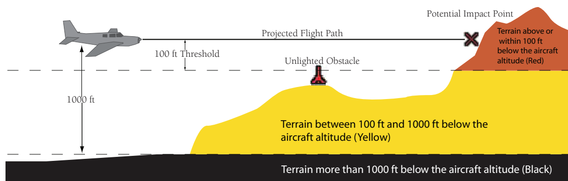
Figure 13-1 Terrain Altitude/Color Correlation for TAWS
